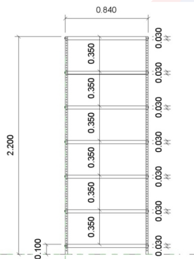
VISTA FRONTAL
